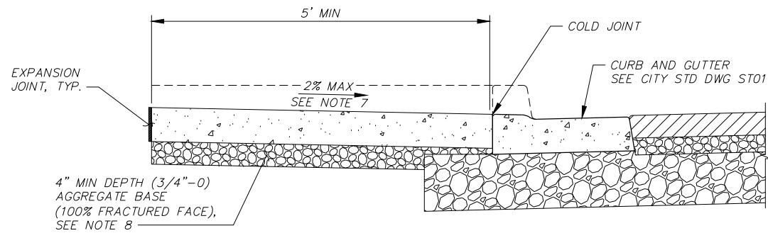
SECTION VIEW
