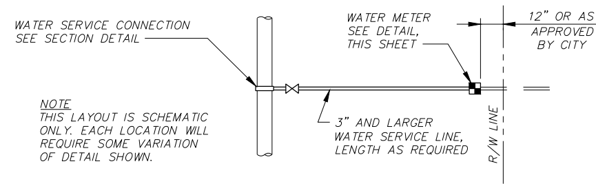
PLAN
