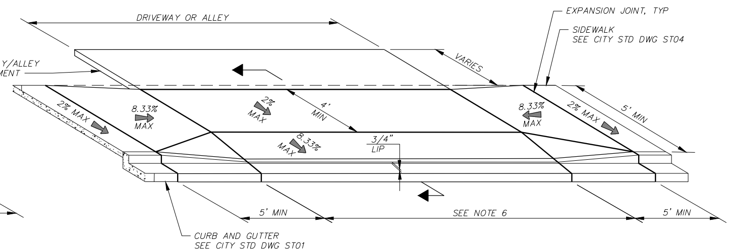
ISOMETRIC VIEW
