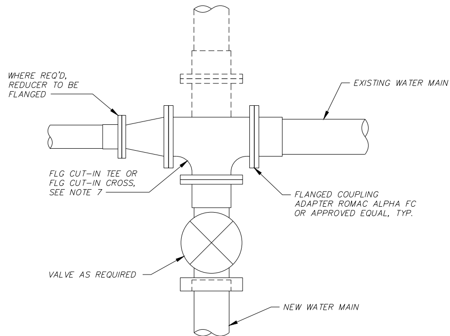
CUT-IN TEE
