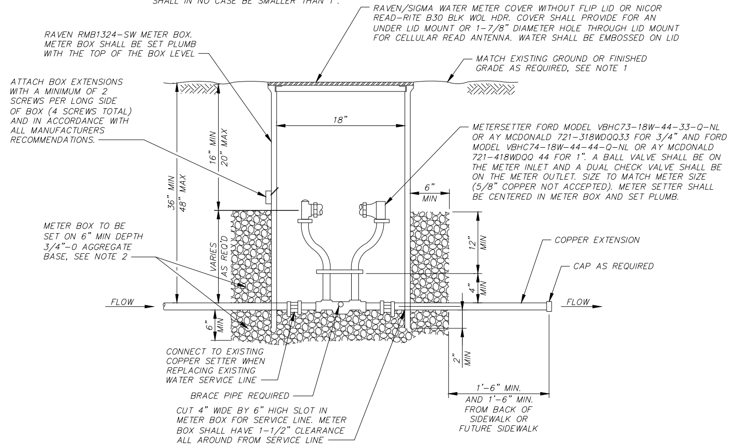
TYPICAL 3/4" OR 1" WATER METER INSTALLATION
