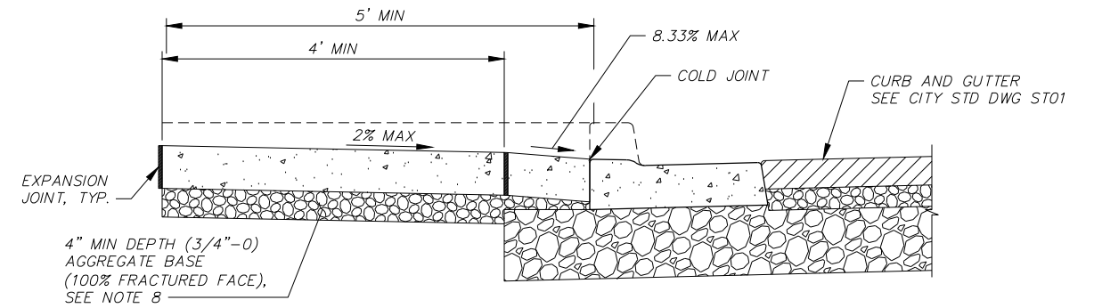
SECTION VIEW
