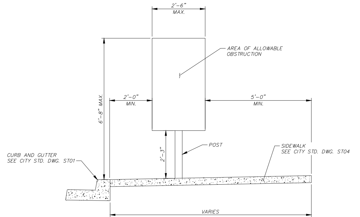
POST MOUNTED OBSTRUCTION WITHIN SIDEWALK
