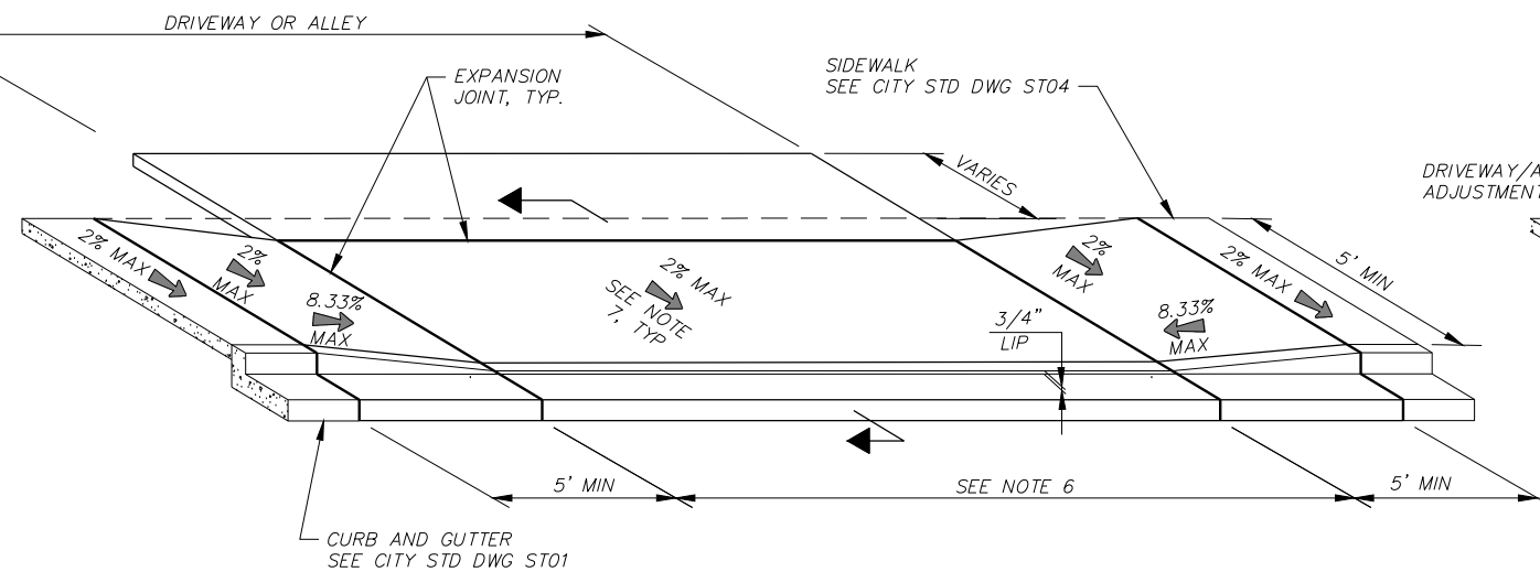
ISOMETRIC VIEW
