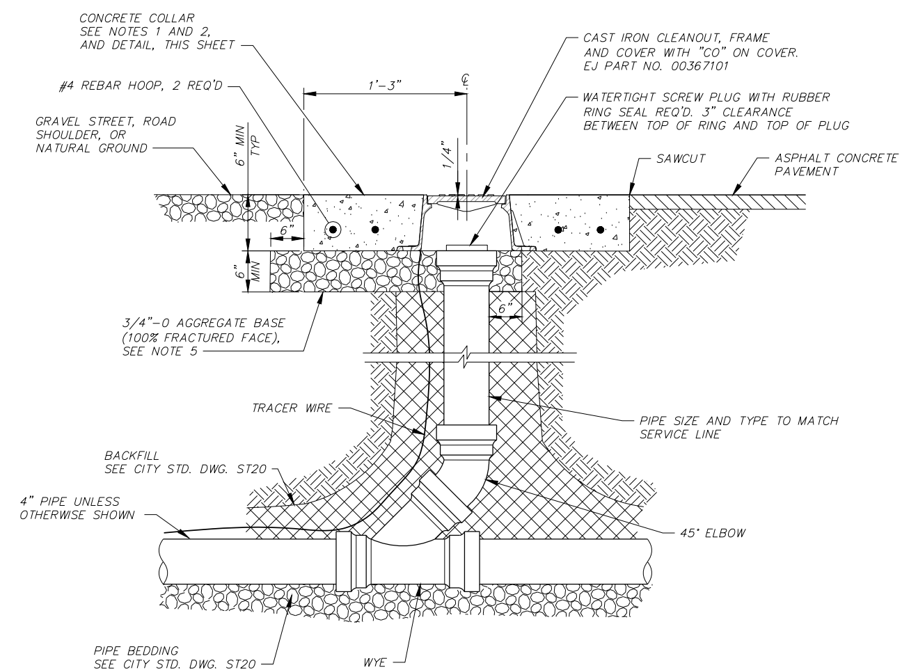
SEWER SERVICE LINE CLEANOUT
