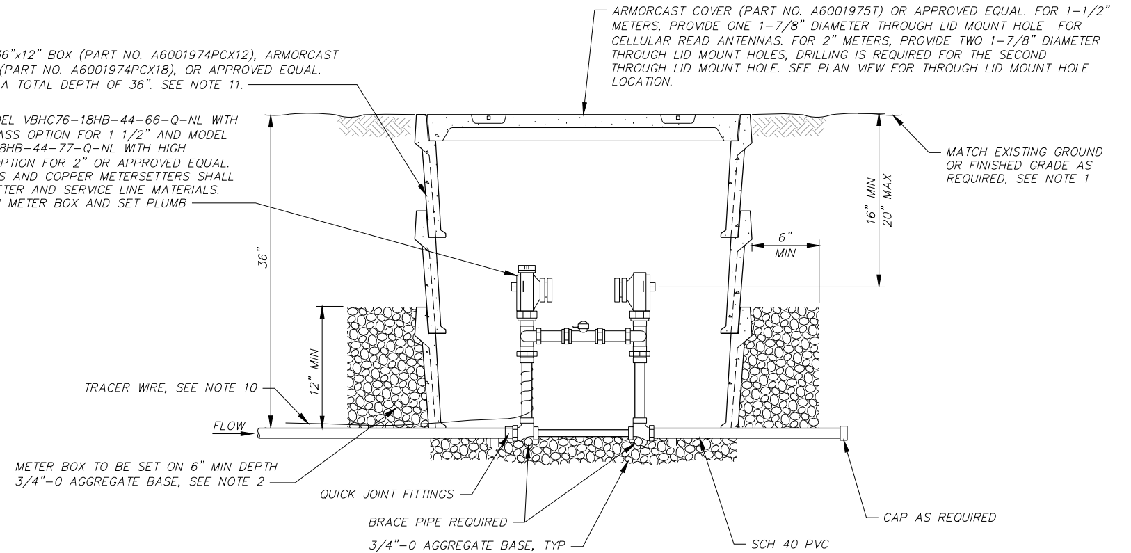
TYPICAL 1-1/2" OR 2" WATER METER INSTALLATION
