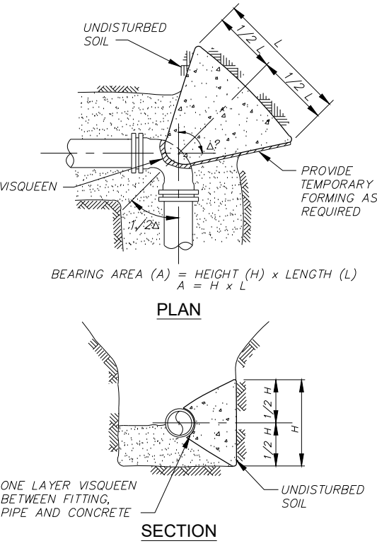
TYPICAL THRUST BLOCK DETAILS
